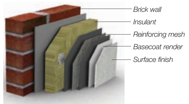
An external wall insulation system
